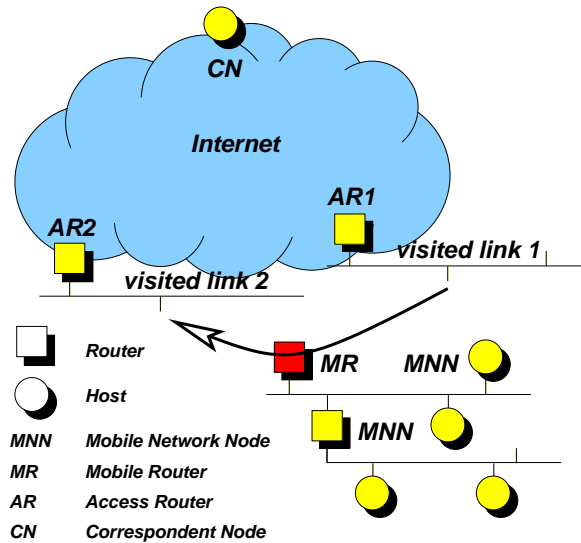
Fig. 1. NEMO Terminology
