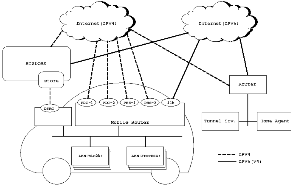
Fig. 3. InternetCAR Testbed
